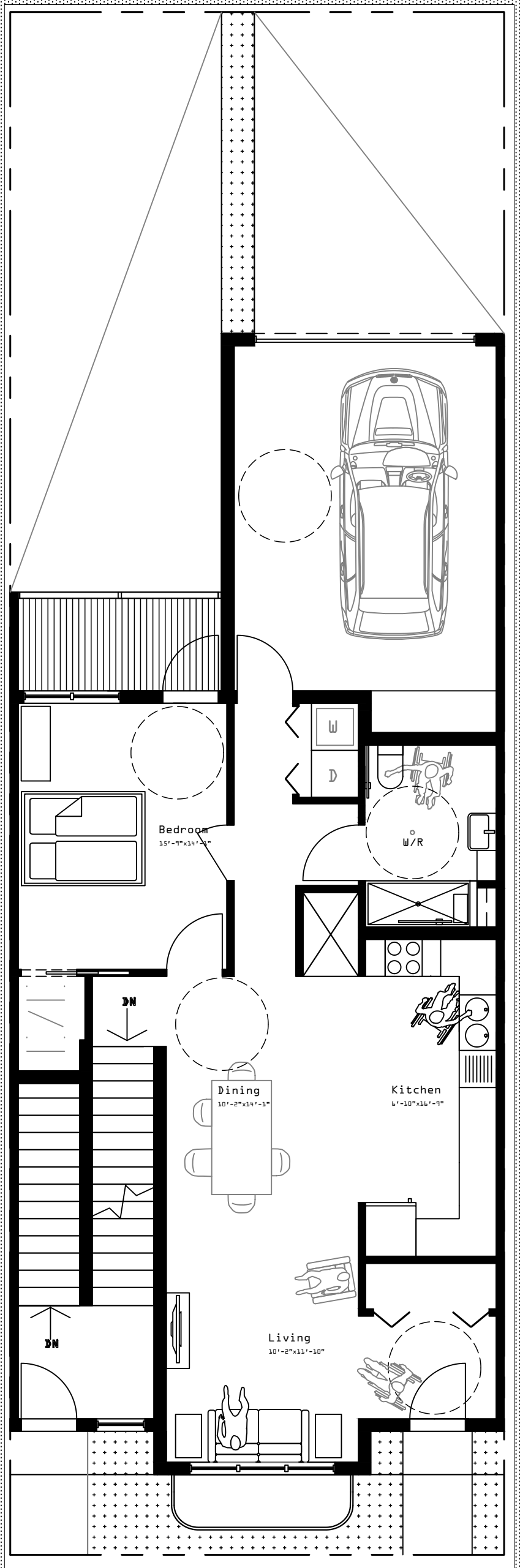
A Ground Level 1-1 Scale 1:75
